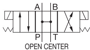
OPEN CENTER
