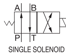
SINGLE SOLENOID
