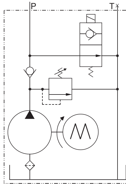
"S5-S8, P5-P8" CIRCUIITS
