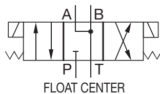
FLOAT CENTER
