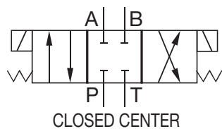
CLOSED CENTER
