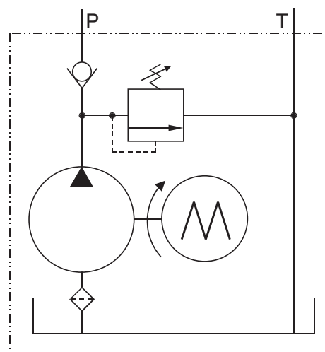
"SW" CIRCUIIT
